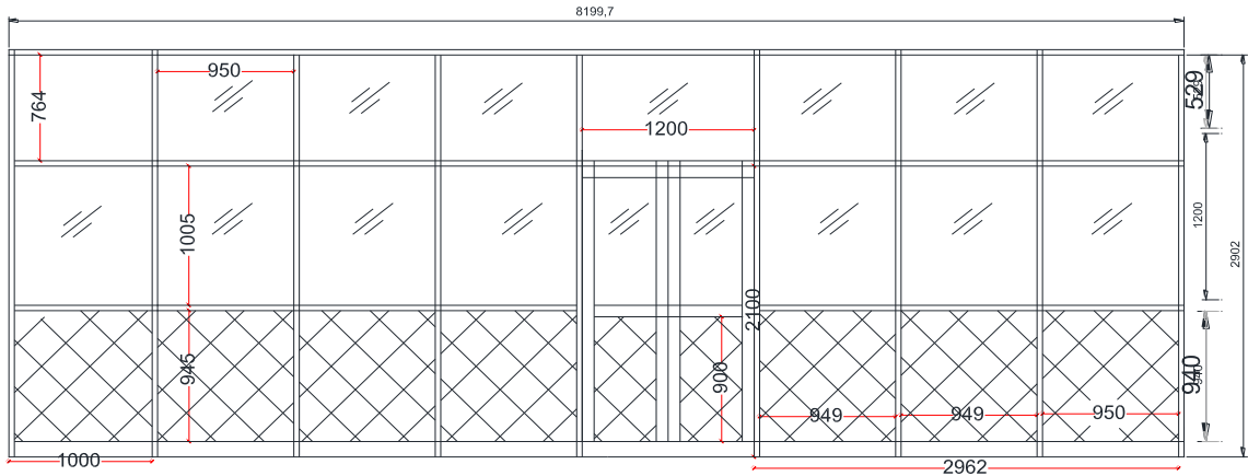
Aluminum Partition, Class Room, 1st floor BBB Building
