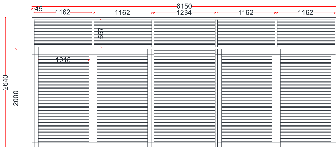
Ele panel AI ventilation partition
